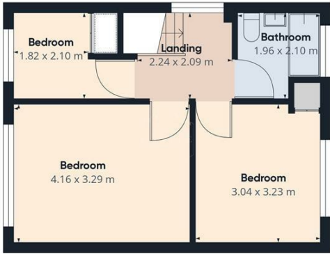
Floor 1 Building
